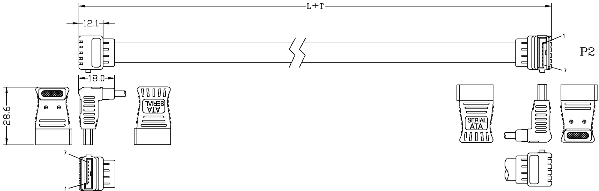
P2 SERIAL ATA 7PIN PLUG
