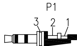
DC3.5 STEREO PLUG
