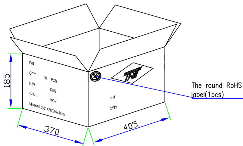
Outer Carton
