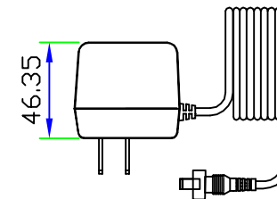
Power adapter Input: AC110-240V Output: DC5V, 2.0A
