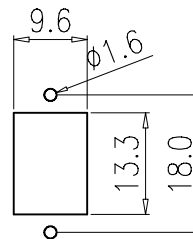
SUGGESTED PANEL CUTOUT
