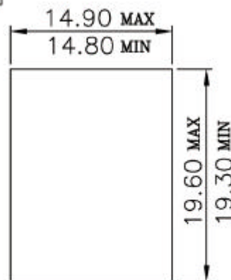
Single Panel-Latch Clearance Panel Thickness 0.062 inch
