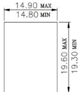
Single Panel-Latch Clearance Panel Thickness 0.062 inch
