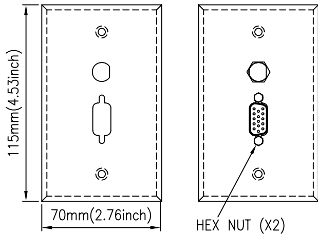
HDB15+3.5F FACEPLATE
